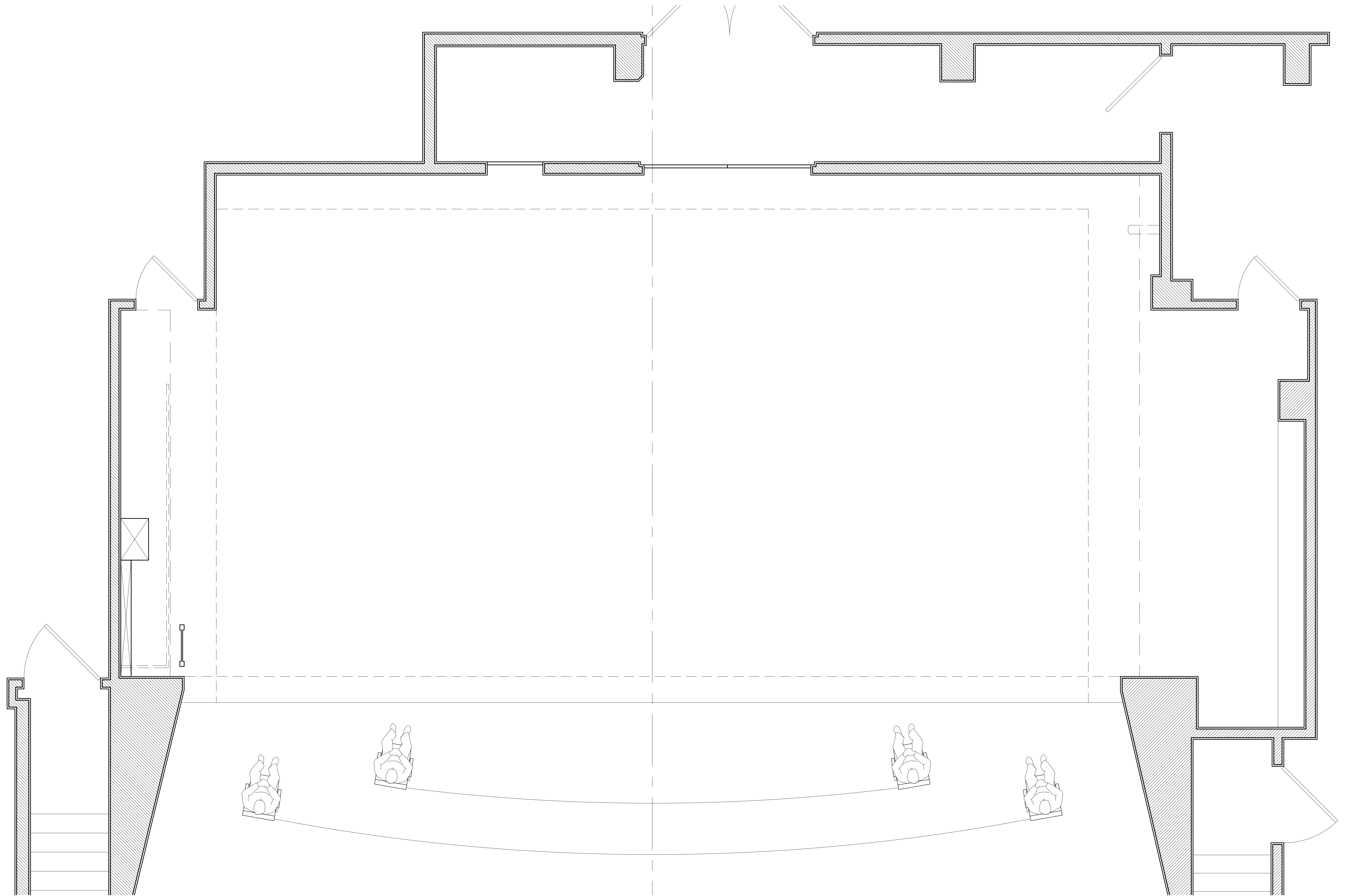
STAGE 3: PLAN VIEW SCALE: 1/2" = 1'-0"
